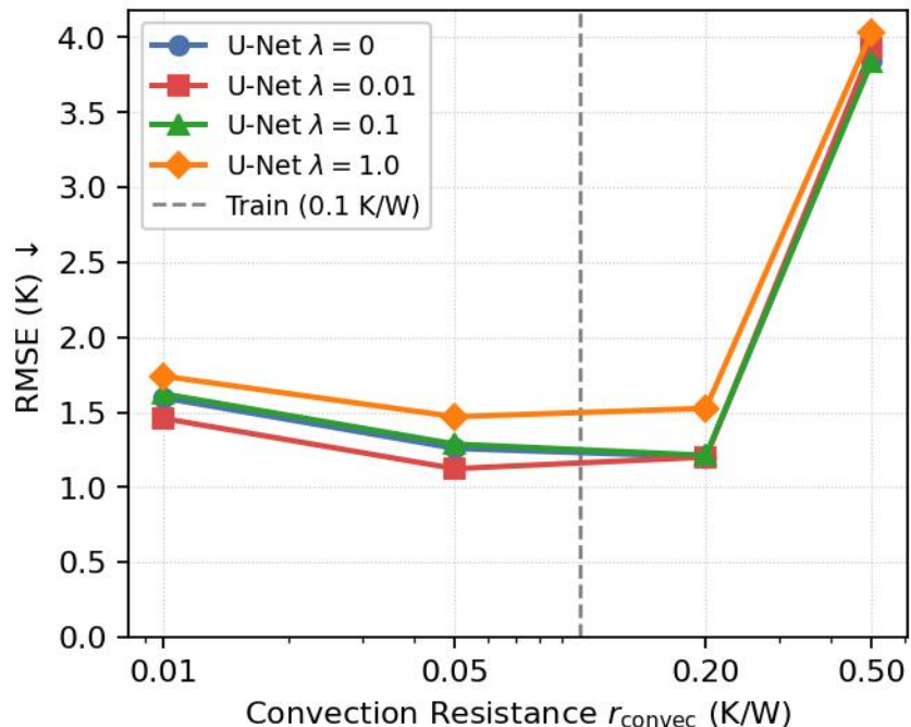
OOD: Convection Resistance
